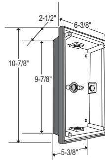
2 1/2" Cast Aluminum Backbox/Surface Conduit (CSTB)
