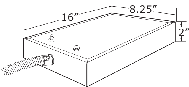
Box 8.25" W x 16"L x 2"H is used for following Remote Emergency Batteries: REM5, REMC2, REMC4, REMH1, REMH3, REMH4
