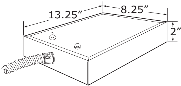
Box 8.25"W x 13.25"L x 2"H is used for following Remote Emergency Batteries: REM1, REM2, REMC1, REMC3
