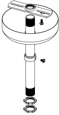
ST12 = 12" Stem (1/2" Dia.) w/ Static Canopy
